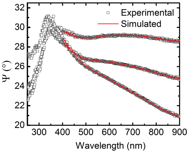
FIG. 2. Measured (black squares) and simulated (red lines) ellipsometric spectra of ultra-thin (~2.0 nm) plasma-grown titanium oxide films at three different angles of incidence (65°, 70°, and 75°). By fitting the measurement data to the Cauchy model, the oxide thickness was calculated.
