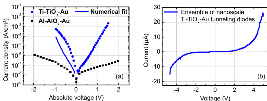
FIG. 3. (a) Measured (blue circles) and simulated (blue lines) current-voltage characteristics of a shadow-mask-patterned microscale Ti-TiO x -Au and Al-AlO x -Au (black squares) tunneling diode. (b) Measured current-voltage-characteristics of an ensemble of transfer-printed nanoscale Au-TiO x -Ti tunneling diodes.
